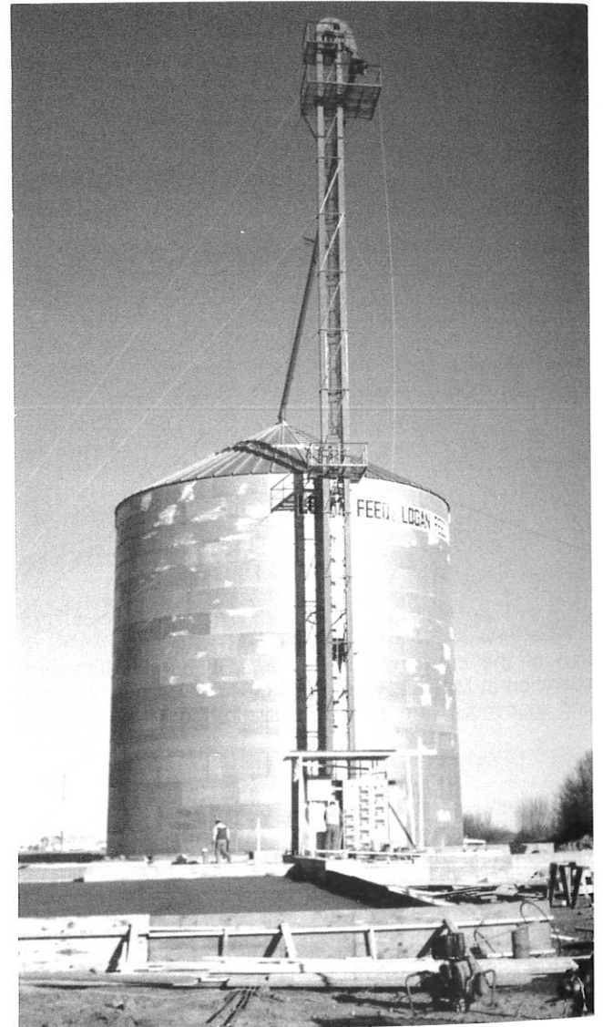
Setting up new "Pea Processing Plant" by rail in Legal, Alberta. New storage bin with a capacity of 160,000 bushels, with a 5000 bushel per hour grain leg - 150 feet long with 135 feet above ground. Will be able to load directly onto rail cars. Plans also in place to split peas for domestic and export requirements.
