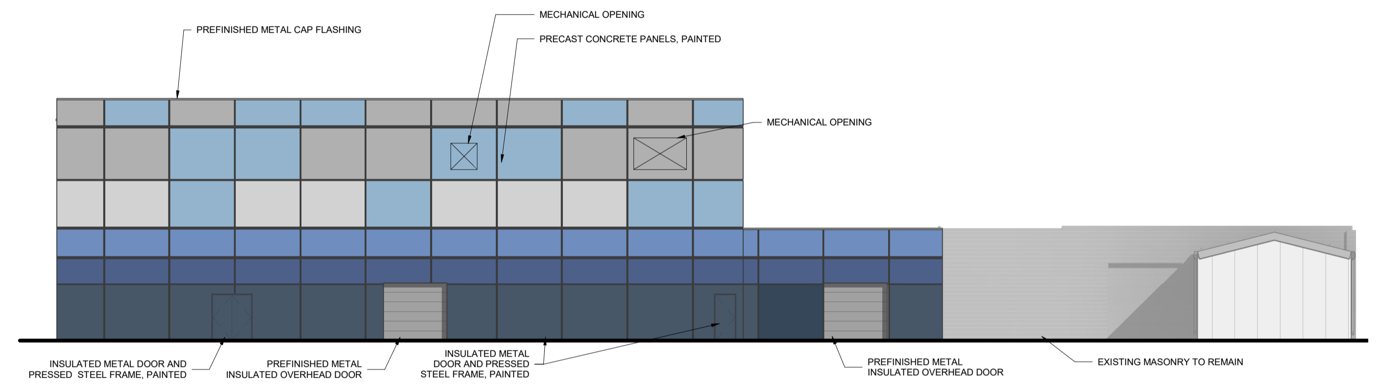
NORTH ELEVATION
