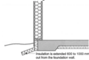
Slab On Grade - Engineered Structural Slab
