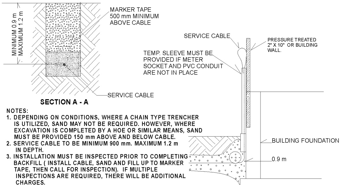
CABLE DETAIL IF NO METER SOCKET.
